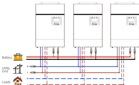
PARALLEL CONNECTION
